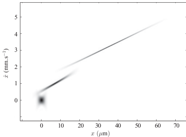
FIG. 3. Wigner function of the wave function at different times t/\tau = 0, 4.5 , and 7 for f(t) = e^{-t/\tau} with \tau = 10 ms. The wave function is evolved according to the 1D Gross-Pitaevskii wave function with an initial condition corresponding to the Thomas-Fermi regime ( Ng_1 = 53 \hbar^{3/2} \omega_0^{1/2} m^{-1/2} ).
